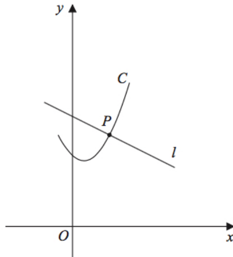
Figure 6: x = 2 \tan t + 1, y = 2 \sec^2 t + 3
