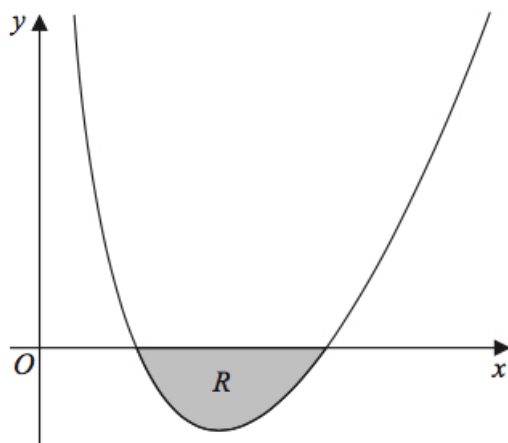
Figure 3: y = \frac{(x-2)(x-4)}{4\sqrt{x}}, \quad x > 0
