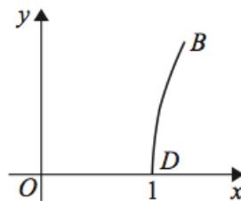
Figure 2: y = \ln(3.6x - k)
